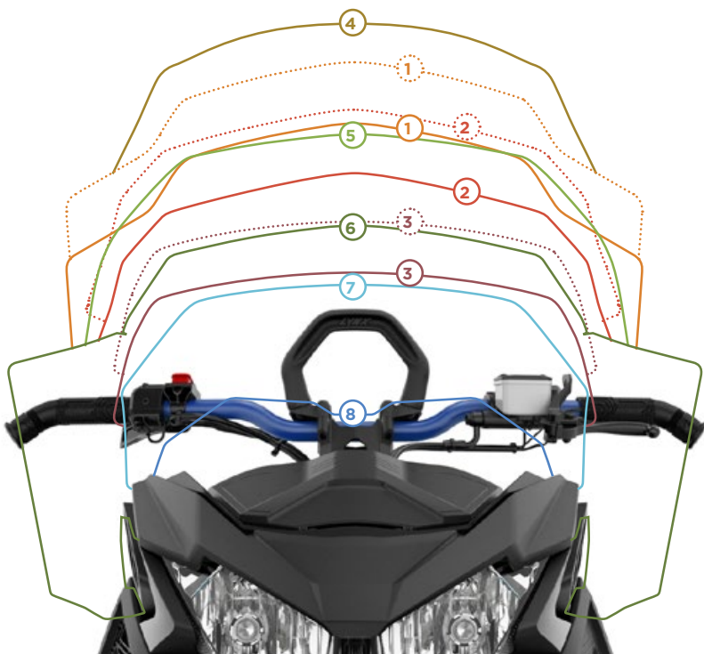
WINDSHIELD, LOW 860202262 36 cm high. Includes windshield support. RADIEN / RADIEN-X
